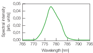
Typical emission spectrum (linear).
