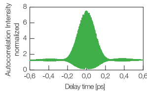
Interferometric autocorrelation.
